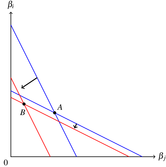
Figure 1: As risk increases, measured by \sigma^2 , both best responses shift inwards. The initial equilibrium is at A while the new equilibrium is at B . The best response of firm j shifts more than that of firm i . As a result, firm i offers stronger incentives, while firm j offers weaker incentives.
