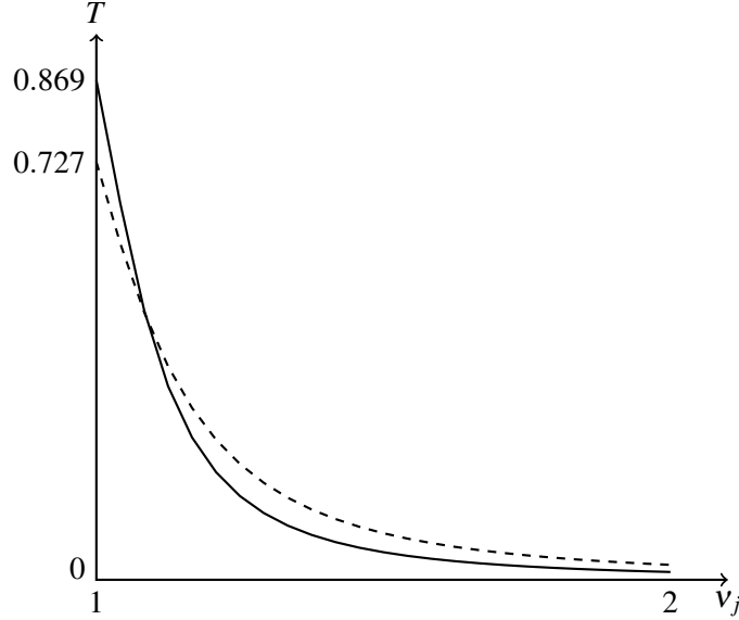
Figure 2: We plot the T curve for two different values of k —the solid curve assumes k = 1.4 and the dashed curve assumes k = 1.5 —against the cost of incentivizing the agents. For any v_j , where v_j \equiv 1 + kr_j\sigma^2(1 - \rho^2) , and a risk aversion asymmetry, \frac{r_i}{r_j} , above T , we have \frac{d\beta_i^*}{d\sigma^2} < 0 and \frac{d\beta_j^*}{d\sigma^2} < 0 , while for a risk aversion asymmetry below T we have \frac{d\beta_i^*}{d\sigma^2} > 0 and \frac{d\beta_j^*}{d\sigma^2} < 0 .
