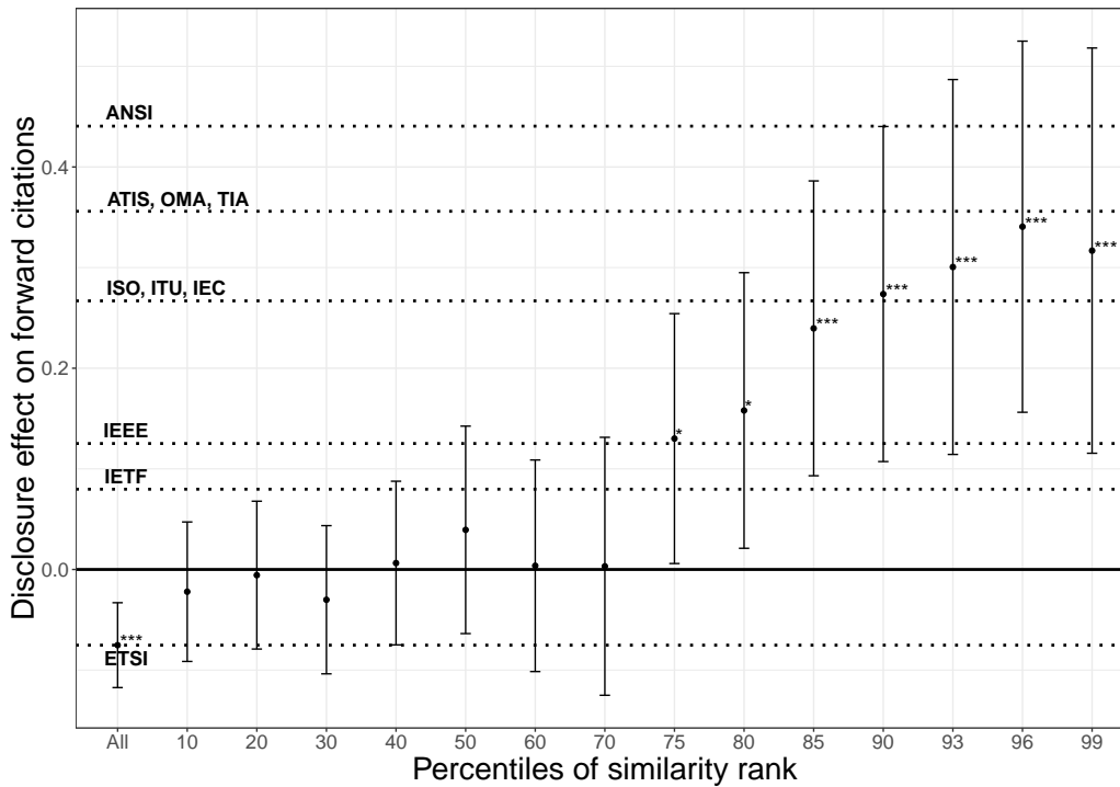
Figure 4: Positive disclosure effects of SEPs at ETSI for the highest ranked SEPs
