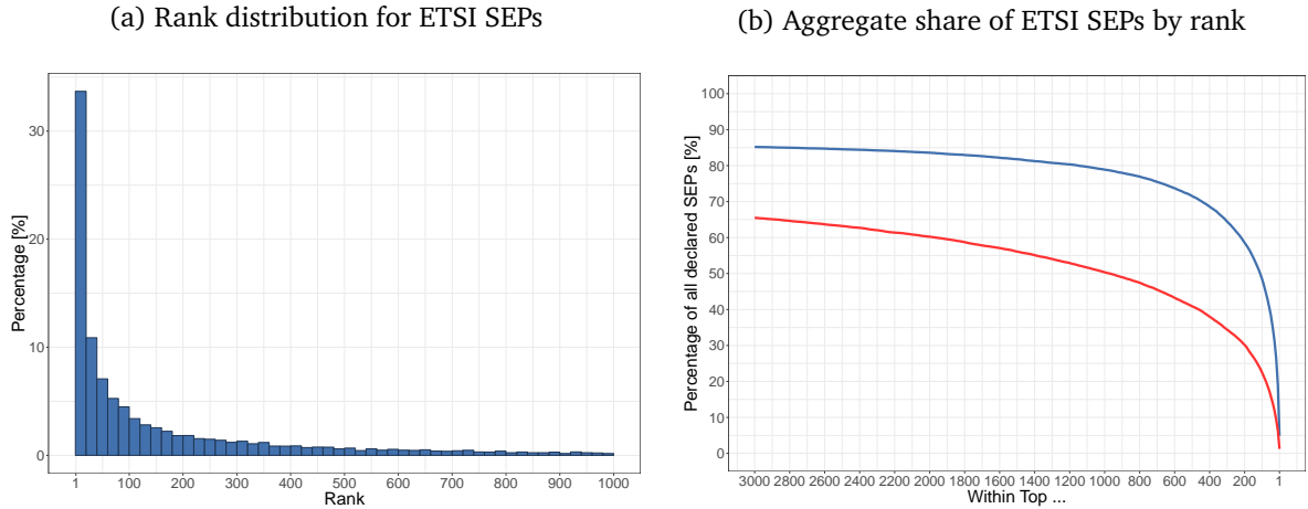
Figure 2: Distribution of SEPs in similarity dataset
