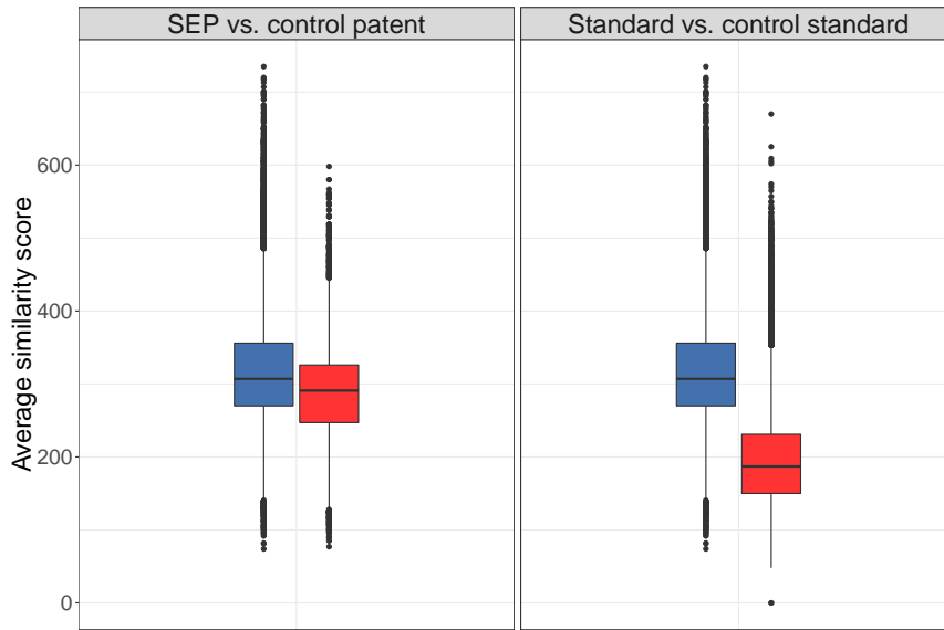
Figure A-3: Comparison of SEP - standard pairs with control groups (censored data)
