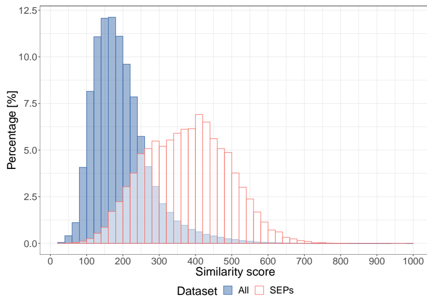
Figure A-2: Similarity score distribution: All patents vs. SEPs
