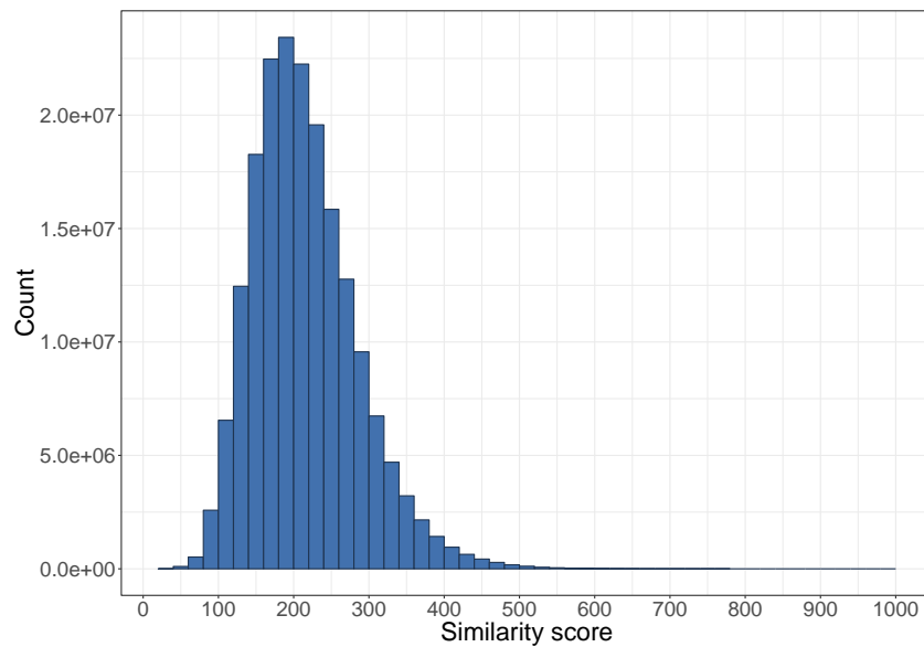
Figure A-1: Similarity score distribution over all standard documents
