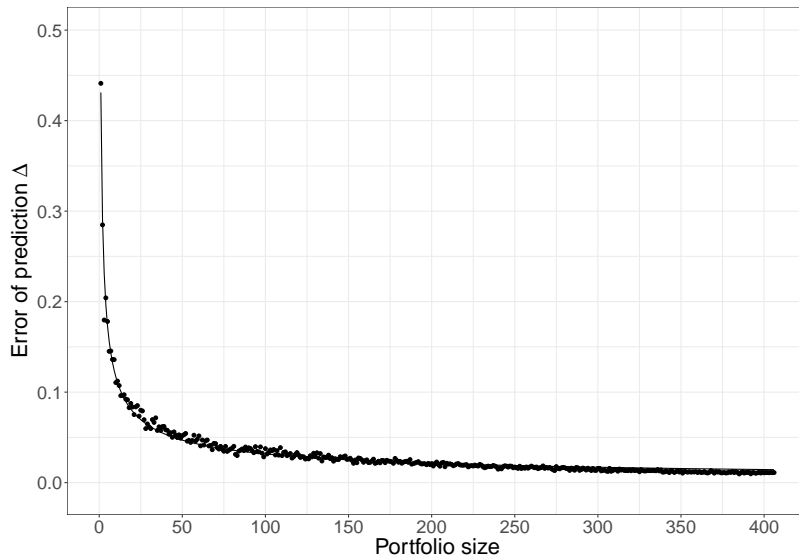
Figure 5: The error of prediction as a function of portfolio size (LTE)
